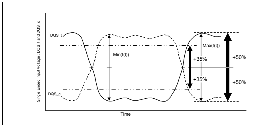
Figure 190 – Definition of differential DQS Peak Voltage and rage of exempt non-monotonic signaling
