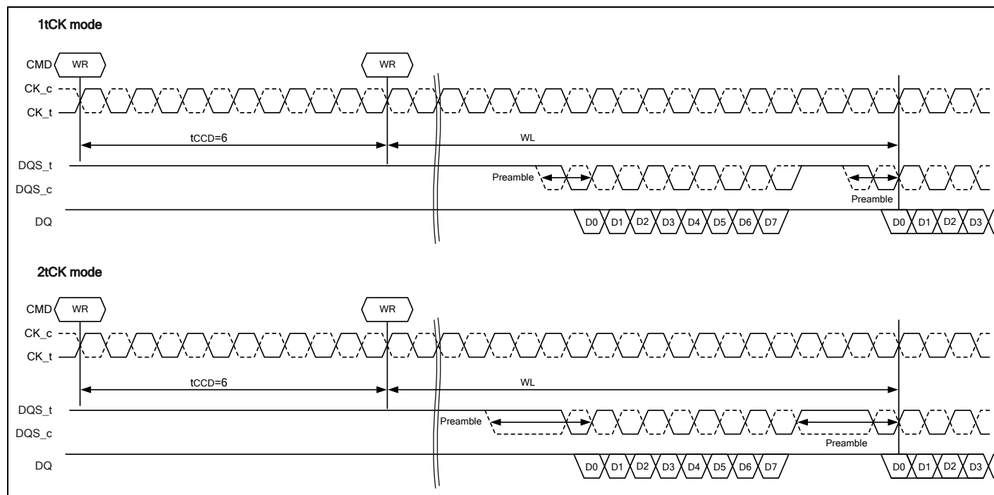
Figure 63 – 1tCK vs. 2tCK WRITE Preamble, tCCD=6 (AL=PL=0)
