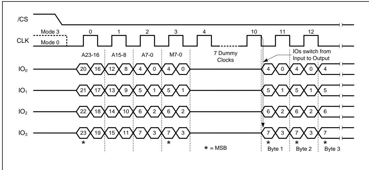
Figure 24b. Fast Read Quad I/O (Previous instruction set M5-4=10, SPI Mode)
