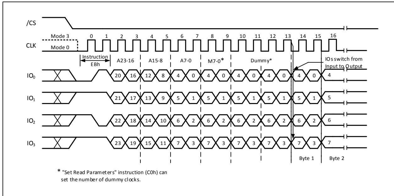
Figure 24c. Fast Read Quad I/O Command (Initial command or previous M5-4≠10, QPI Mode)
