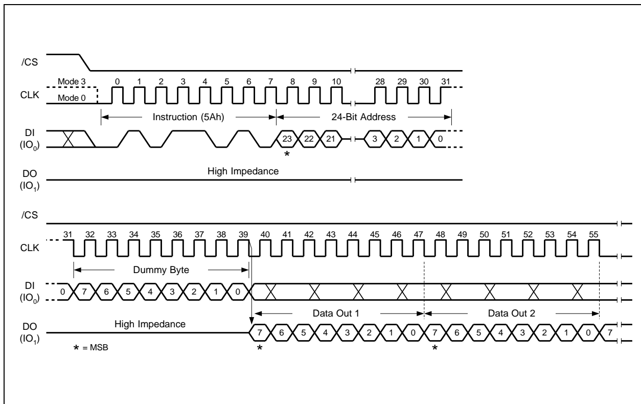
Figure 44. Read SFDP Register Command Sequence Diagram
