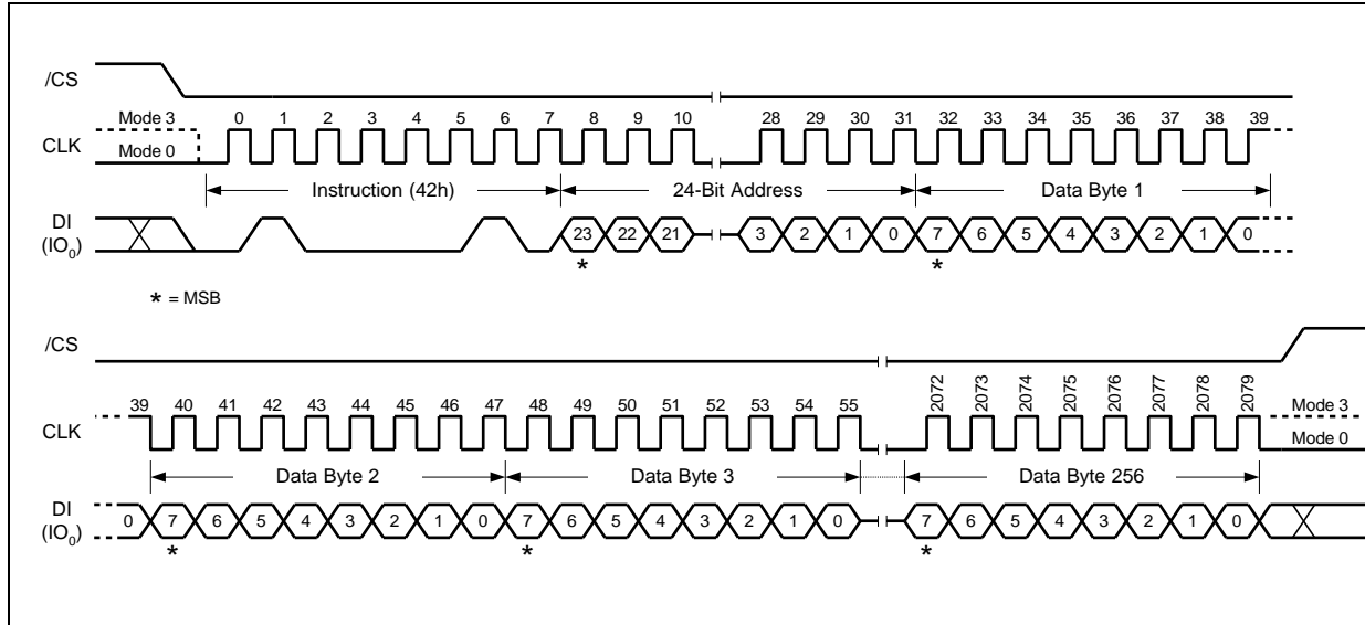
Figure 46. Program Security Registers Command (SPI Mode only)
