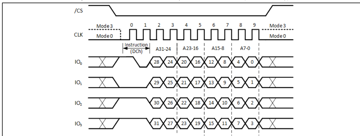
Figure 40b. 64KB Block Erase with 4-Byte Address Instruction (QPI Mode)
