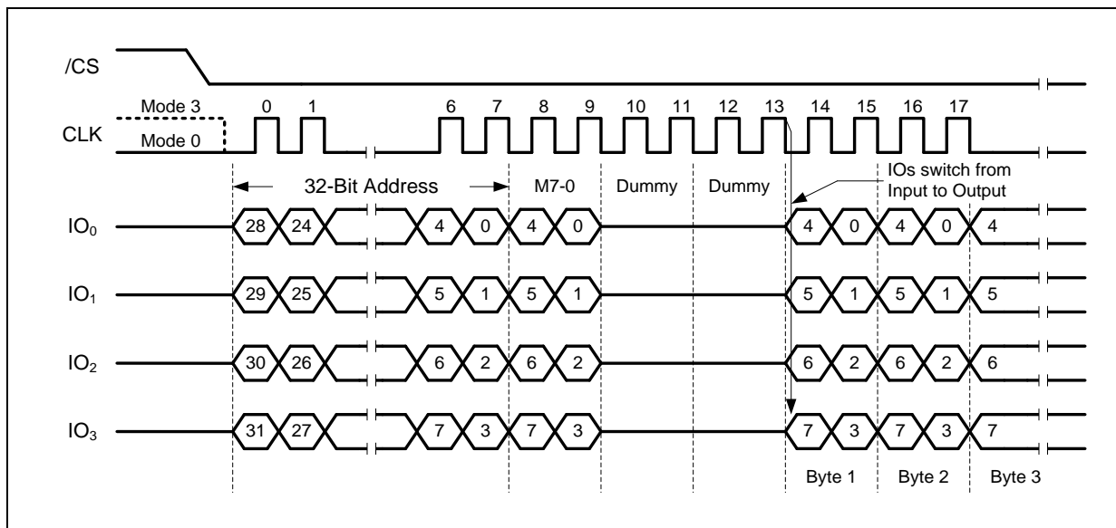
Figure 28b. Fast Read Quad I/O w/ 4-Byte Addr. (Previous instruction set M5-4=10, SPI Mode)
