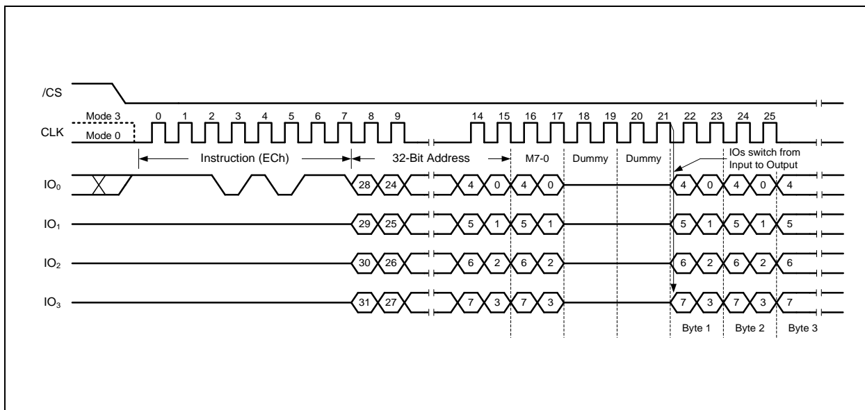
Figure 28a. Fast Read Quad I/O w/ 4-Byte Addr. (Initial instruction or previous M5-4=10, SPI Mode)
