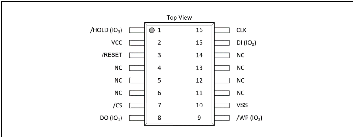
Figure 1b. W25Q25PW Pin Assignments, 16-pin SOIC 300-mil (Package Code SF)
