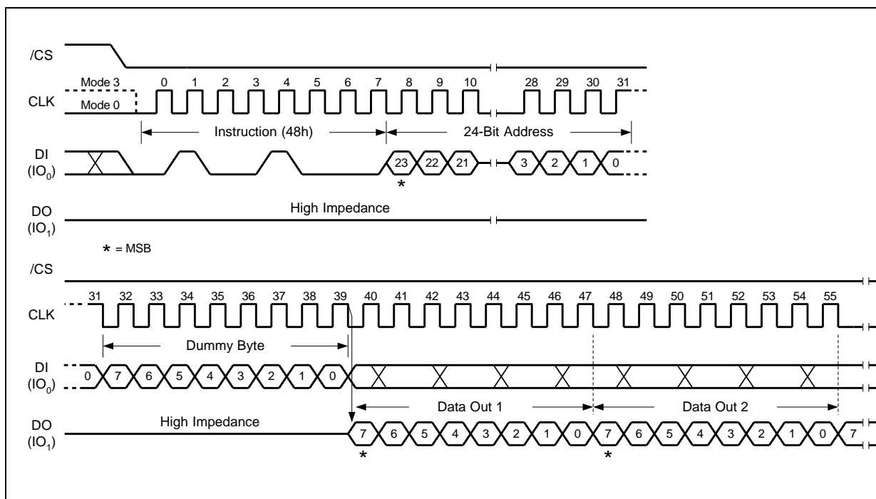
Figure 53. Read Security Registers Instruction (SPI Mode only) 32-Bit Address is required when the device is operating in 4-Byte Address Mode
