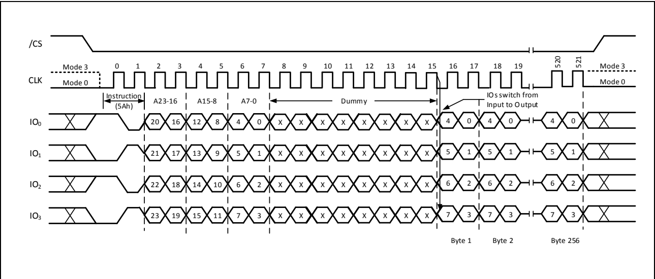
Figure 51. Read QPI Register Instruction Sequence Diagram (QPI Mode) Only 24-Bit Address is required when the device is operating in either 3-Byte or 4-Byte Address Mode
