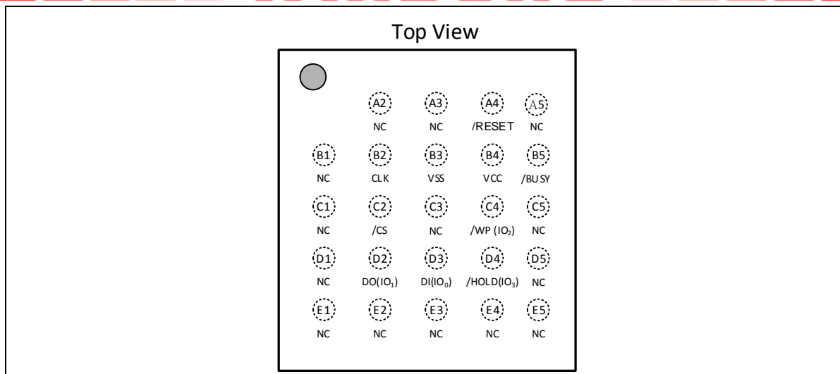
Figure 1c. W25Q25PW Ball Assignments, 24-ball TFBGA 6x8-mm (Package TB)
