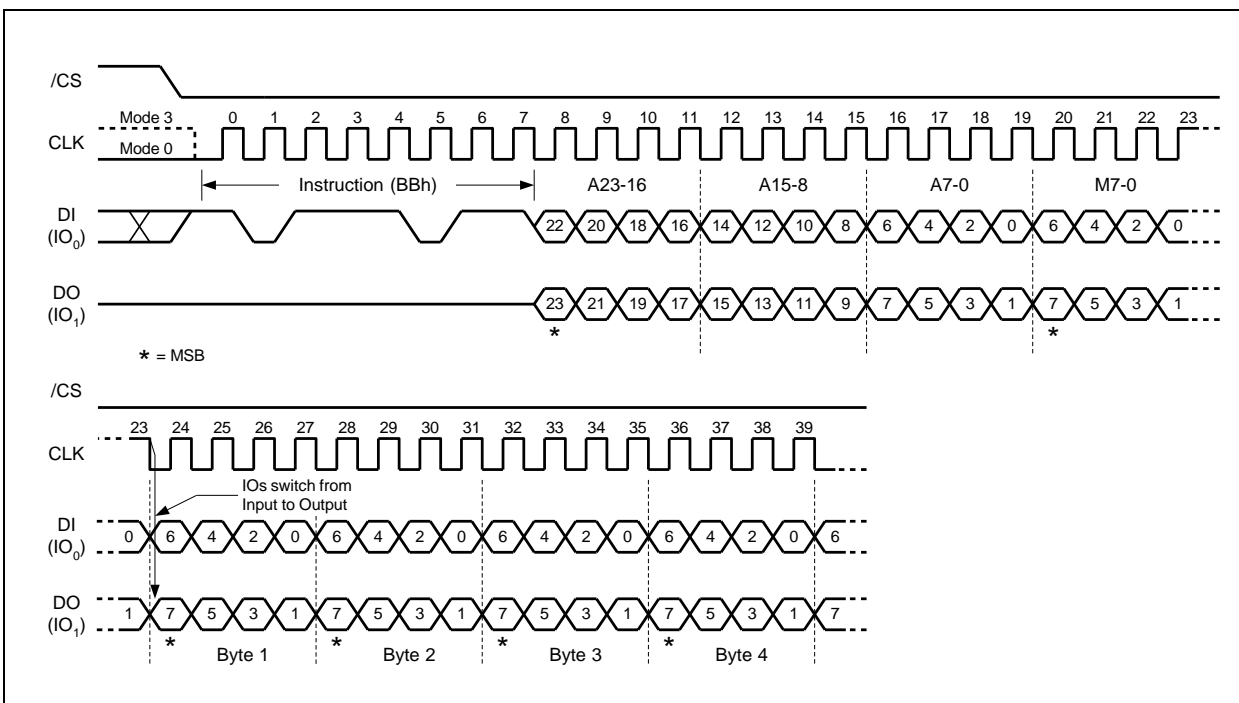
Figure 23a. Fast Read Dual I/O (Initial instruction or previous M5-4≠10, SPI Mode only) 32-Bit Address is required when the device is operating in 4-Byte Address Mode
