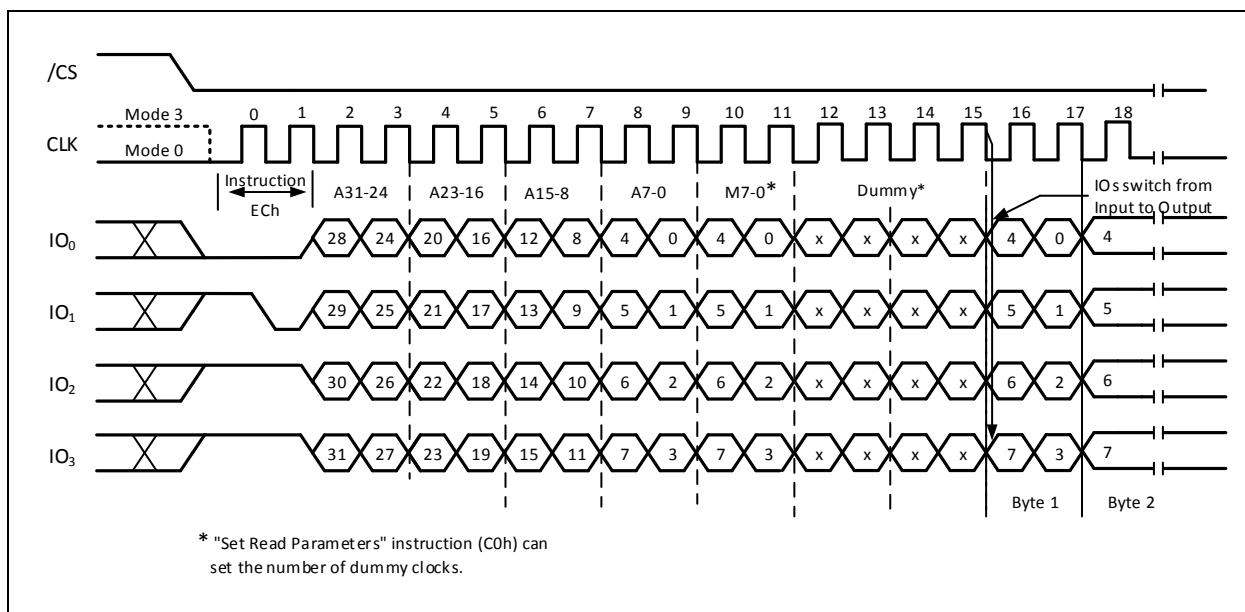
Figure 28c. Fast Read Quad I/O w/ 4-Byte Addr. (Previous instruction set M5-4≠10, QPI Mode)
