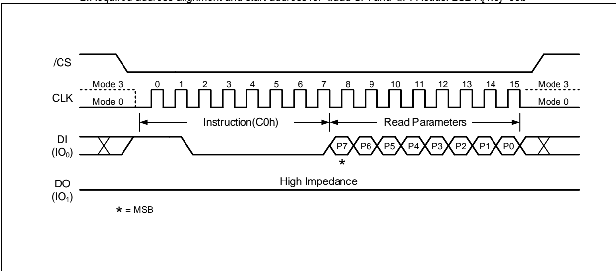
Figure 54a.Set Read Parameters Instruction (SPI Mode)
