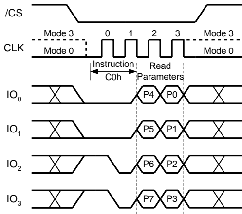
Figure 54b. Set Read Parameters Instruction (QPI Mode)
