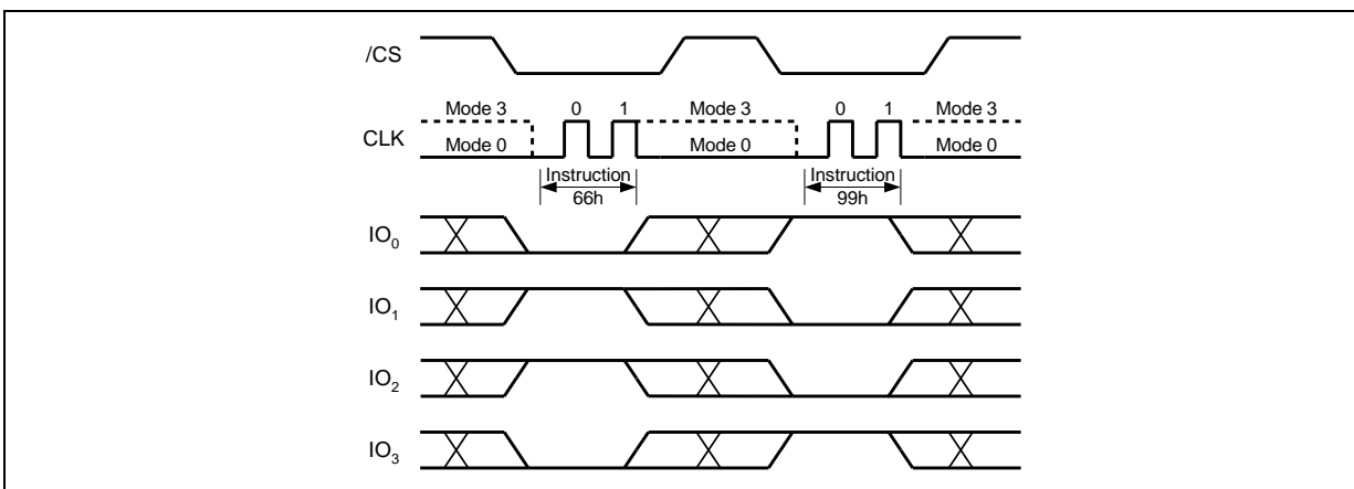
Figure 64b. Enable Reset and Reset Instruction Sequence (QPI Mode)
