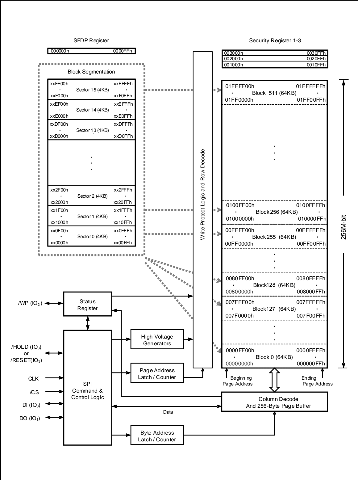
Figure 2. W25Q25PW Serial Flash Memory Block Diagram
