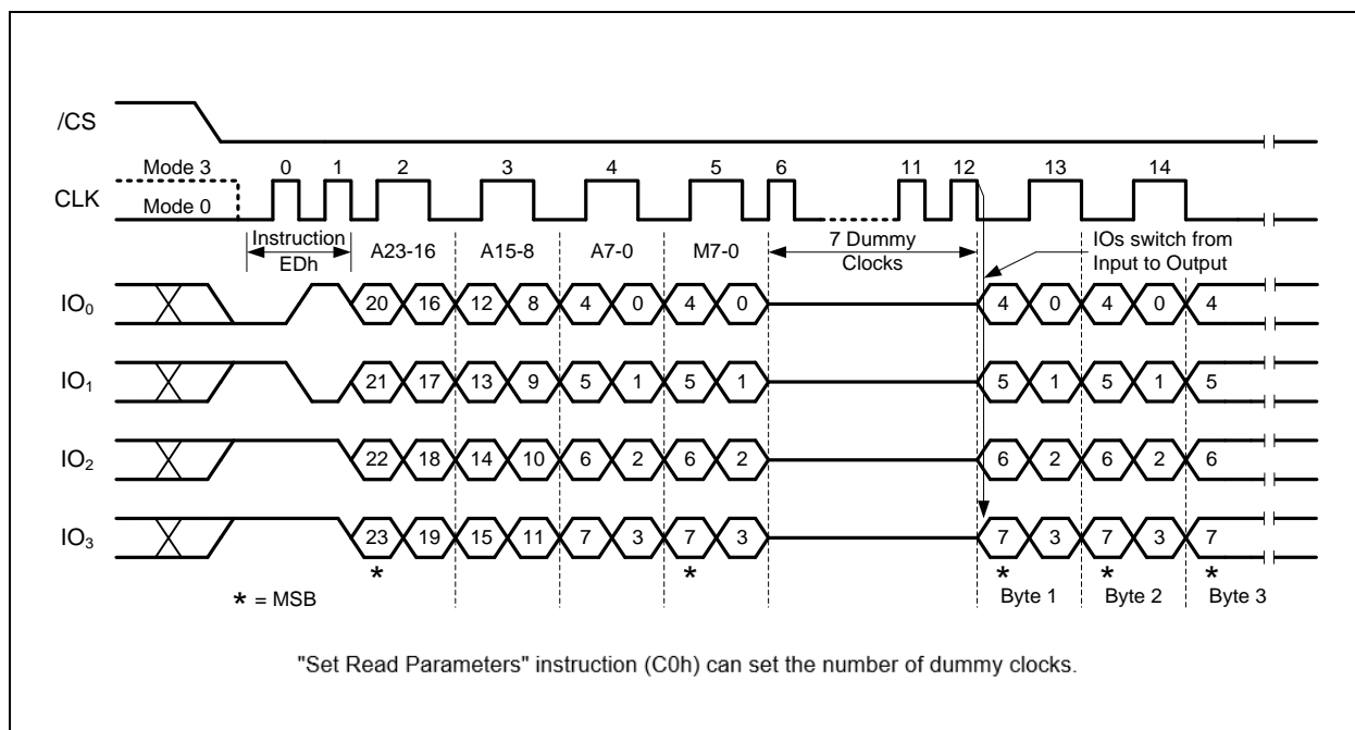
Figure 27c. DTR Fast Read Quad I/O (Initial instruction or previous M5-4≠10, QPI Mode)
