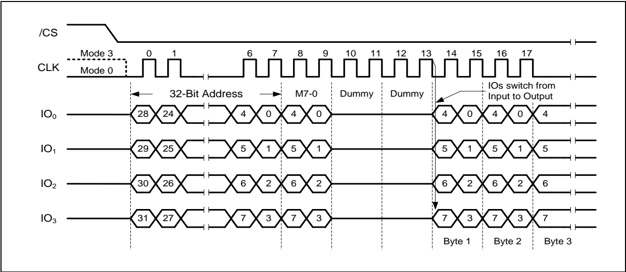
Figure 28b. Fast Read Quad I/O w/ 4-Byte Addr. (Previous instruction set M5-4=10, QPI Mode)
