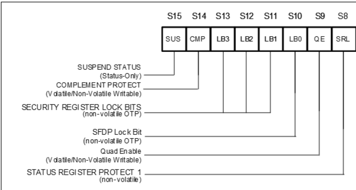
Figure 4b. Status Register-2
