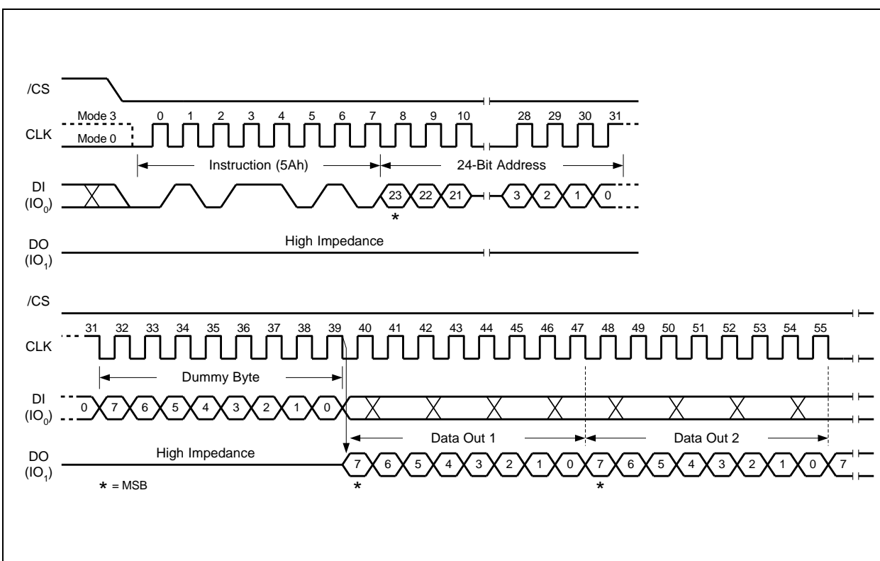
Figure 51. Read SFDP Register Instruction Sequence Diagram (SPI Mode)
