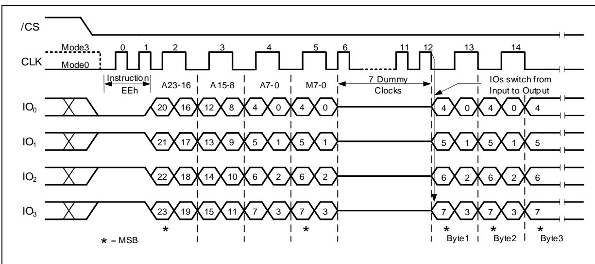
Figure DTR Fast Read Quad I/O with 4-Byte Address (QPI Mode only)
