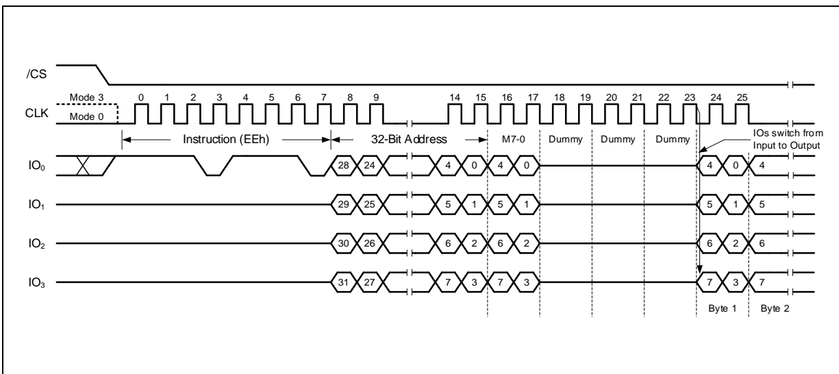
Figure . DTR Fast Read Quad I/O with 4-Byte Address (SPI Mode only)
