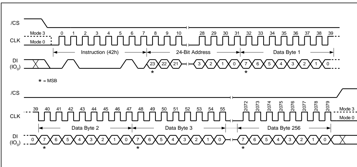
Figure 52. Program Security Registers Instruction (SPI Mode only) 32-Bit Address is required when the device is operating in 4-Byte Address Mode
