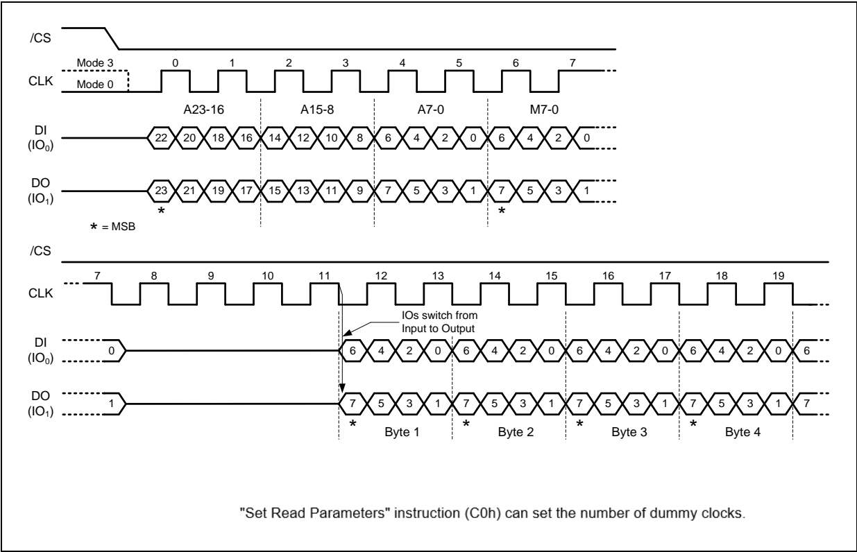
Figure 23b. DTR Fast Read Dual I/O (Previous instruction set M5-4=10, SPI Mode only)
