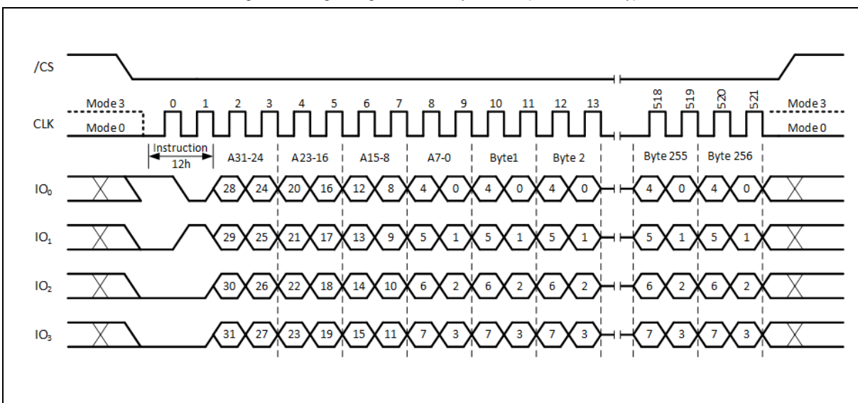
Figure 33b. Page Program Instruction with 4-Byte Address (QPI Mode)
