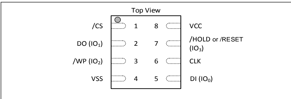
Figure 1a. W25Q25PW Pad Assignments, 8-pad WSON 6x5 & 8x6-mm (Package Code ZP & ZE)
