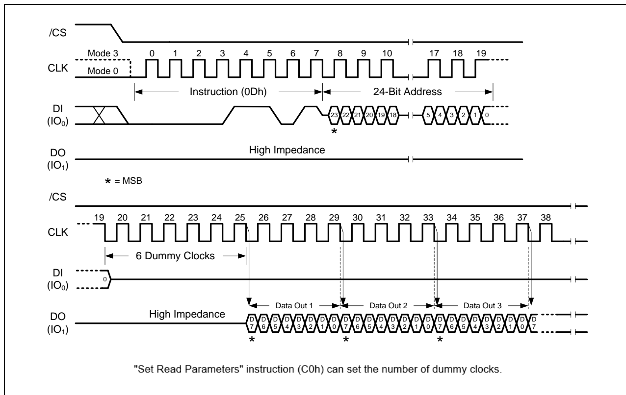
Figure 17a. DTR Fast Read Instruction (SPI Mode)
