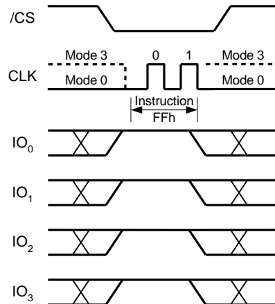
Figure 58. Exit QPI Instruction (QPI Mode only)
