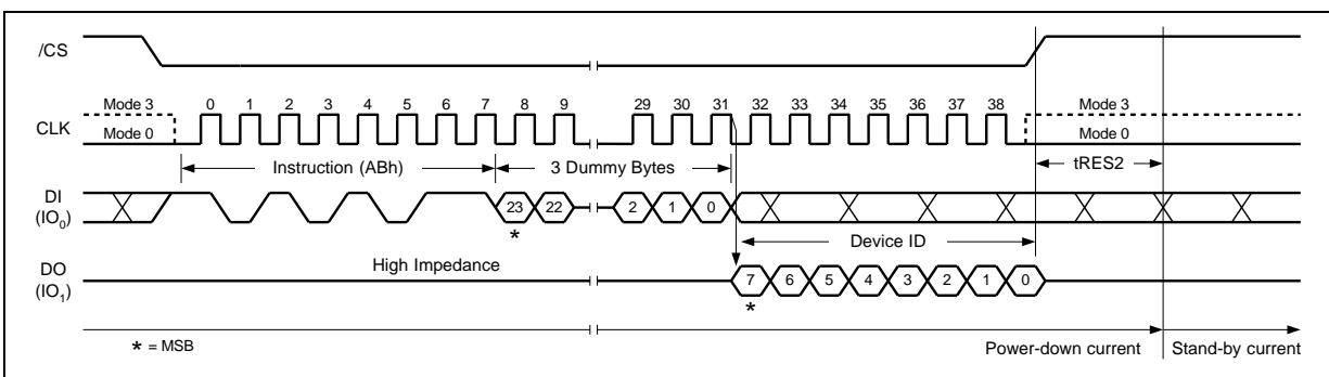
Figure 38c. Release Power-down / Device ID Instruction (SPI Mode)
