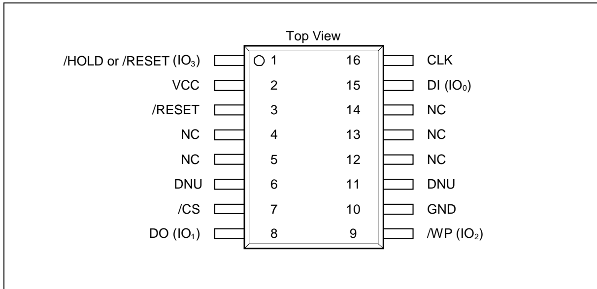
Figure 1b. W25Q512JV Pin Assignments, 16-pin SOIC 300-mil (Package Code F)
