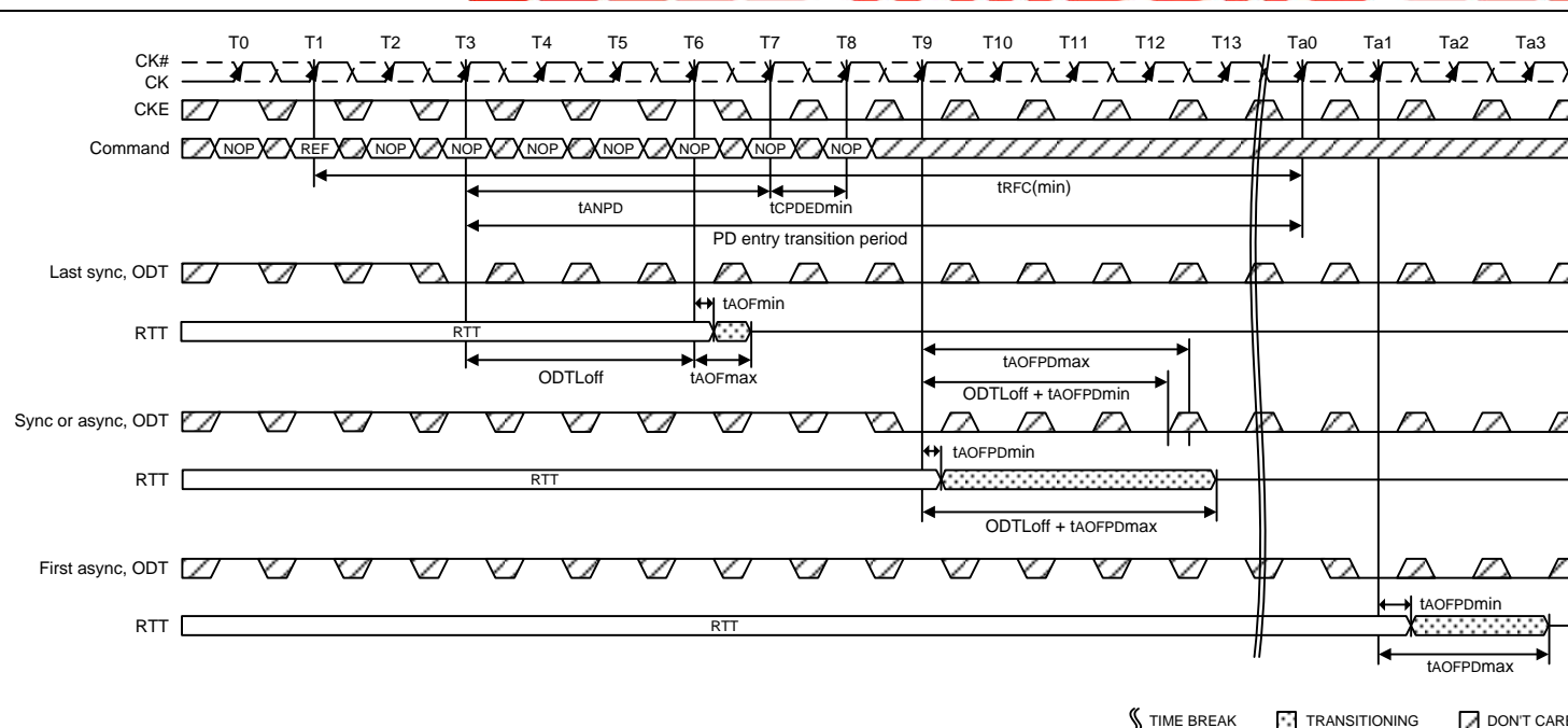
Figure 84 – Synchronous to asynchronous transition after Refresh command (AL = 0; CWL = 5; t_{ANPD} = WL - 1 = 4 )
