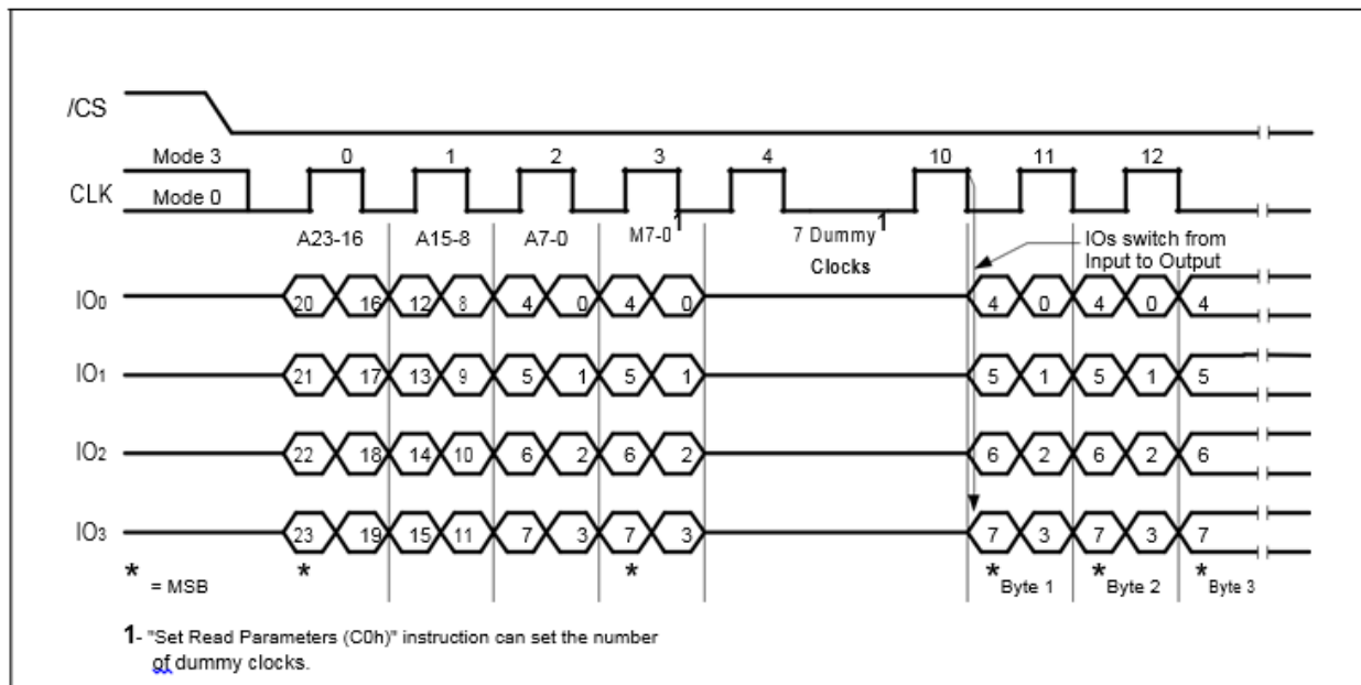
Figure 27d. DTR Fast Read Quad I/O (Previous instruction set M5-4=10, QPI Mode)
