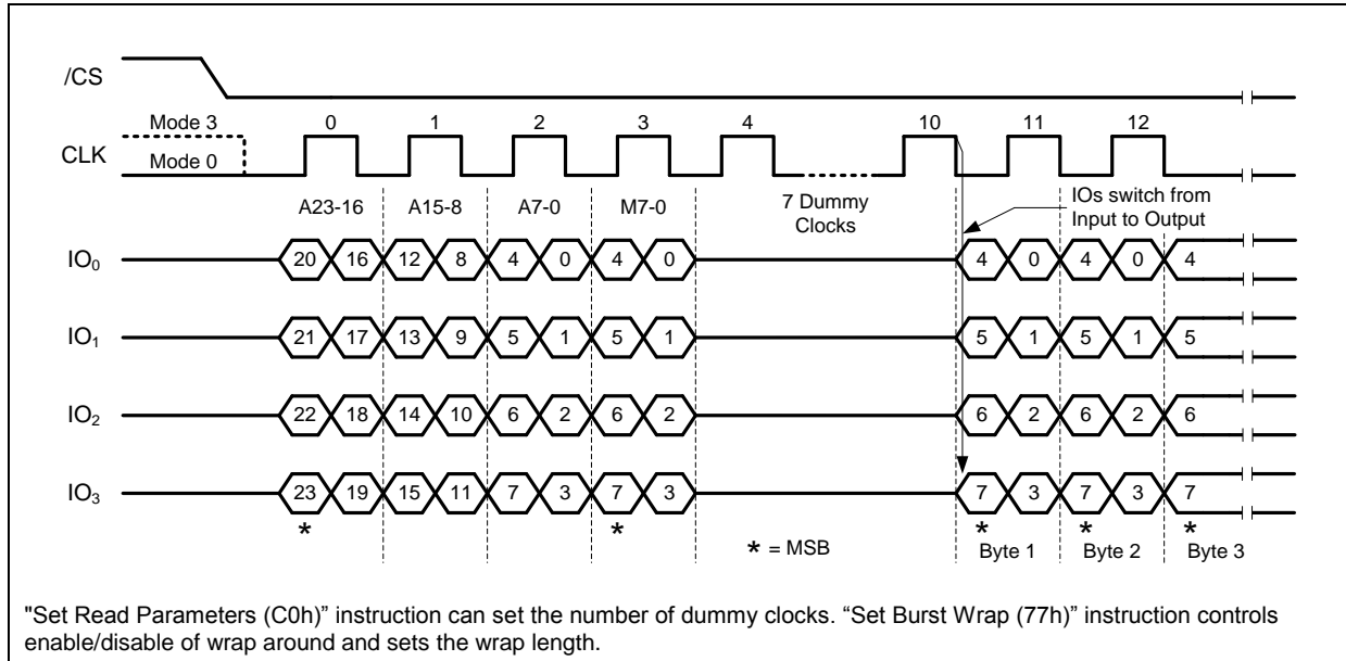
Figure 27b. Fast Read Quad I/O (Previous instruction set M5-4=10, SPI Mode)
