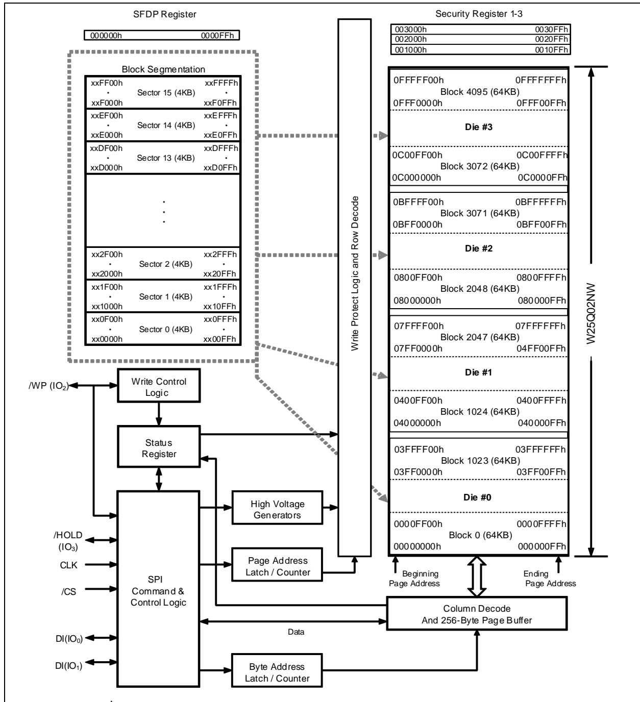
Figure 2. W25Q02NW Serial Flash Memory Block Diagram
