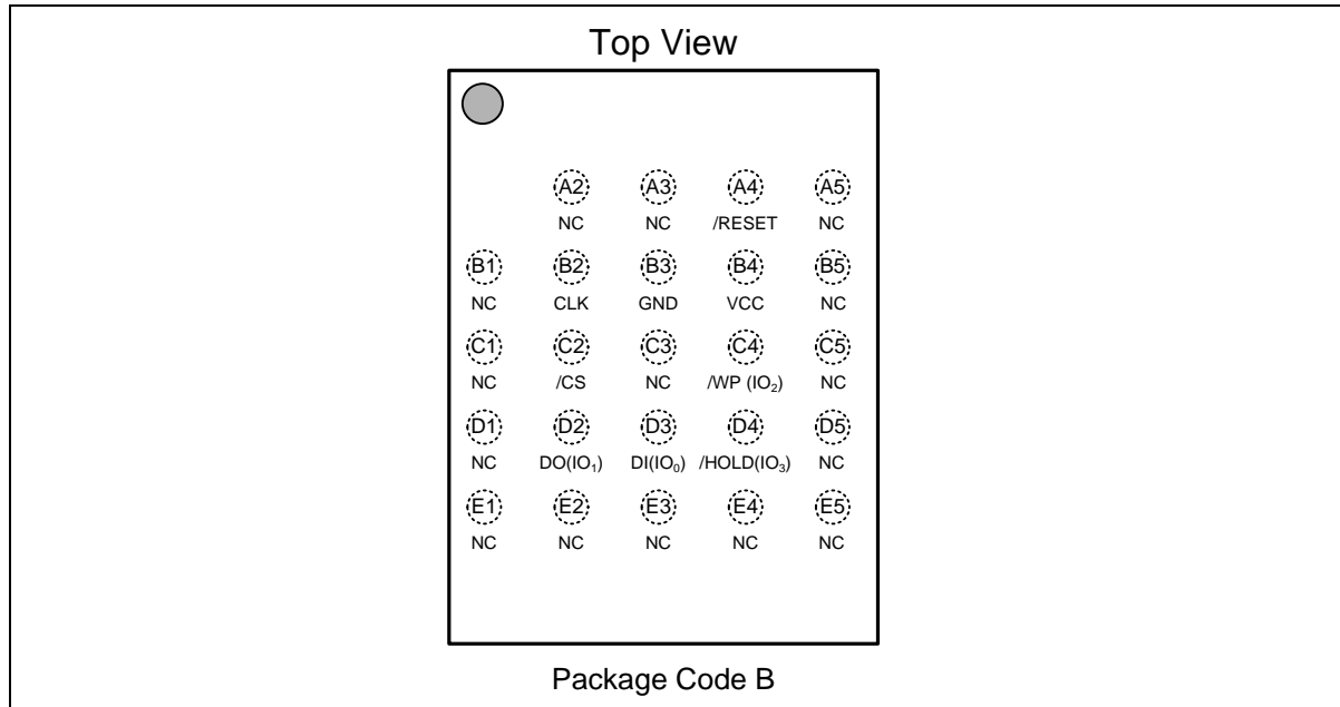
Figure 1c. W25Q02NW Ball Assignments, 24-ball TFBGA 8x6-mm (Package Code TB)
