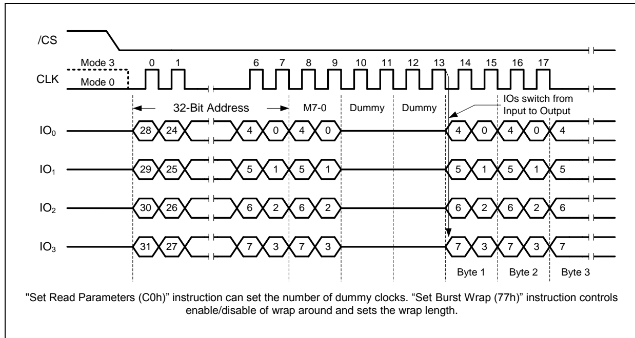
Figure 28b. Fast Read Quad I/O w/ 4-Byte Addr. (Previous instruction set M5-4=10, SPI Mode only)
