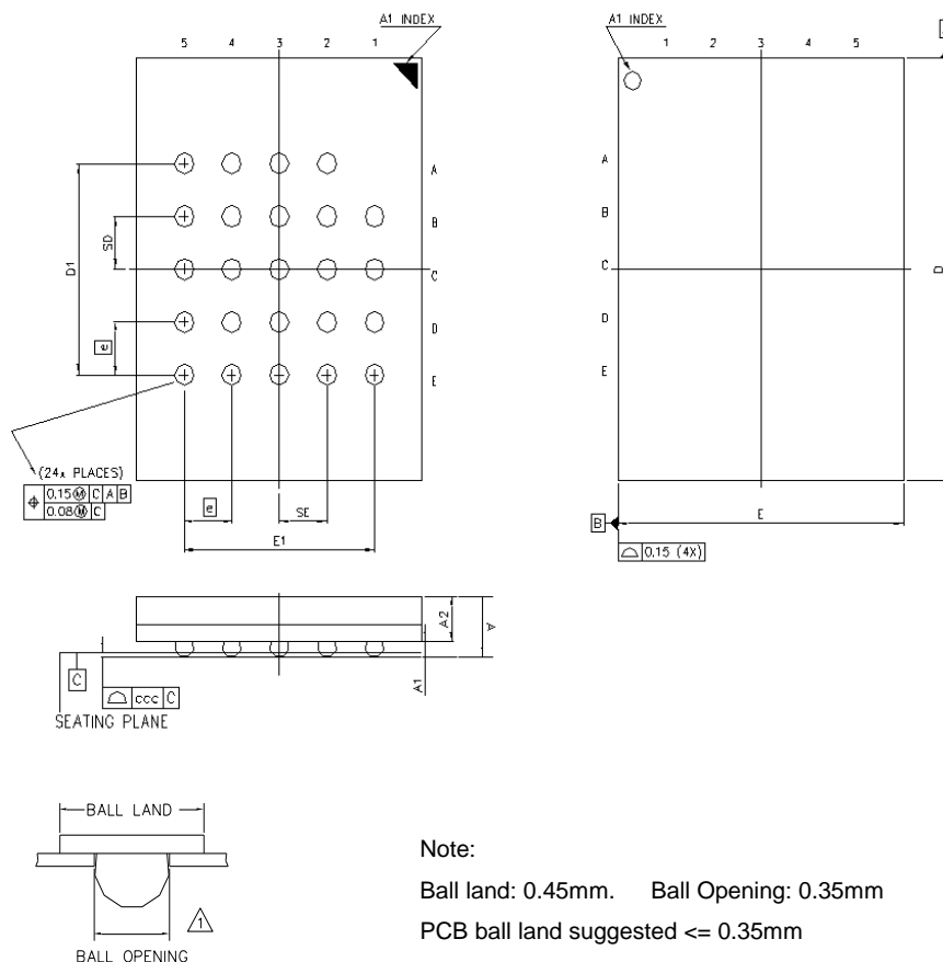
24-Ball TFBGA 8x6-mm (Package Code TB, 5x5-1 Ball Array)
