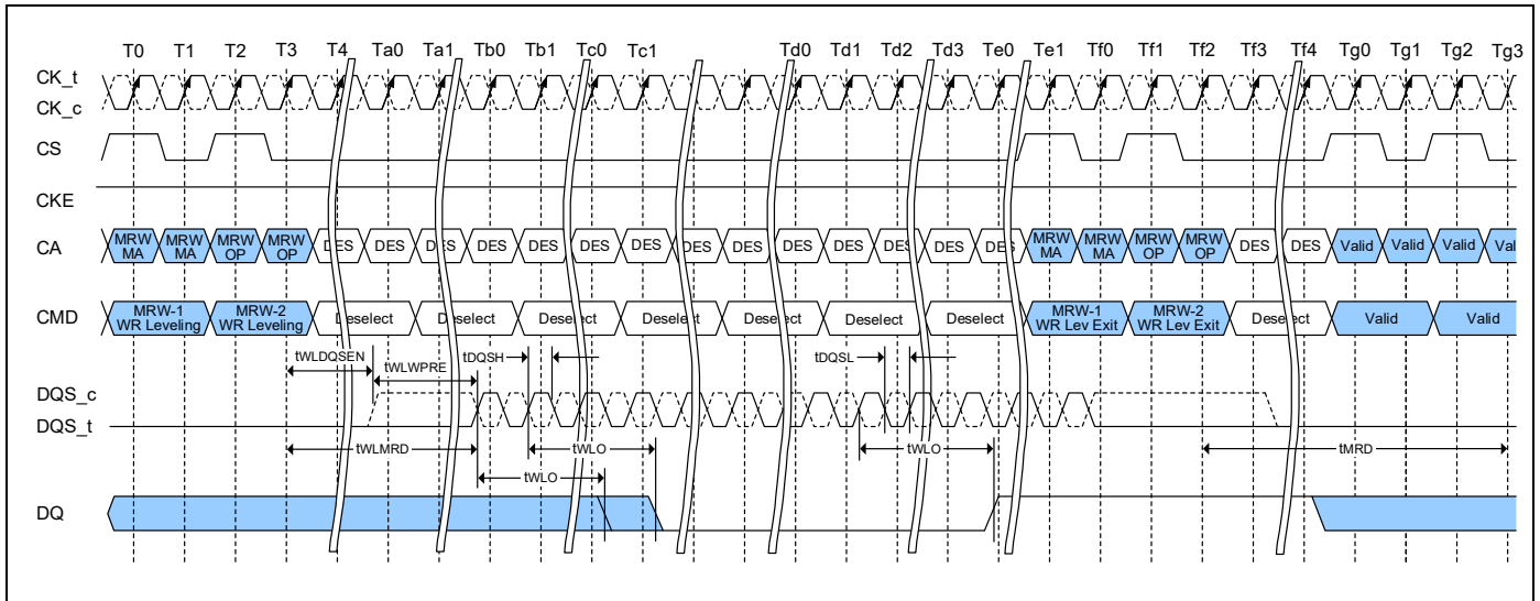
Figure 107 - Write Leveling Timing, t_{DQSL(min)}
