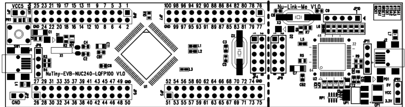
Figure 2-2 NuTiny-SDK-NUC240 PCB Placement
