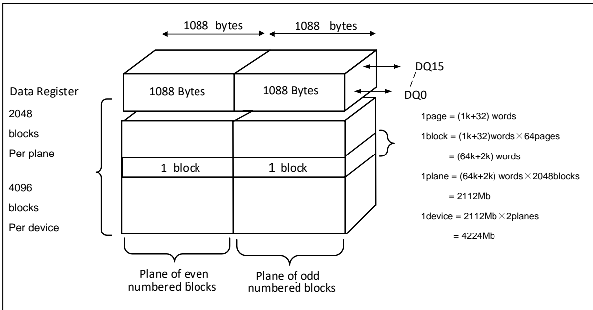
Figure 6-2 Array Organization (x16)
