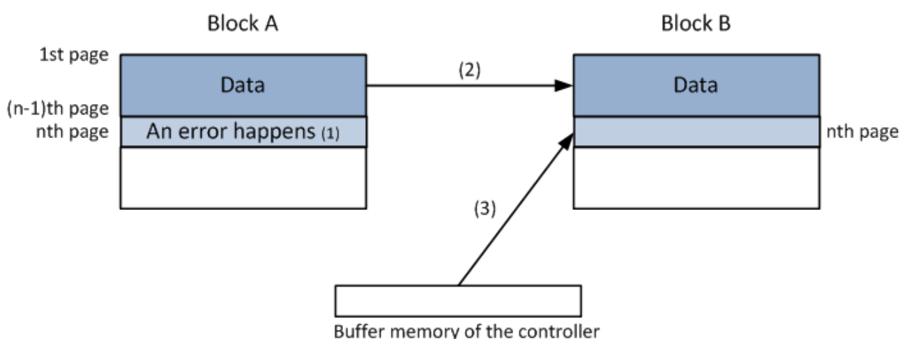
Figure 12-2 Bad Block Replacement
