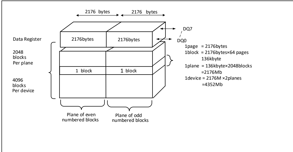
Figure 6-1 Array Organization (x8)
