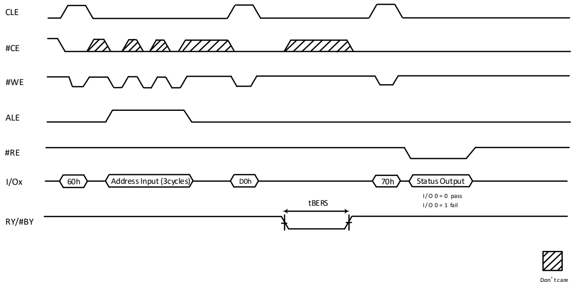
Figure 9-17 Block Erase Operation
