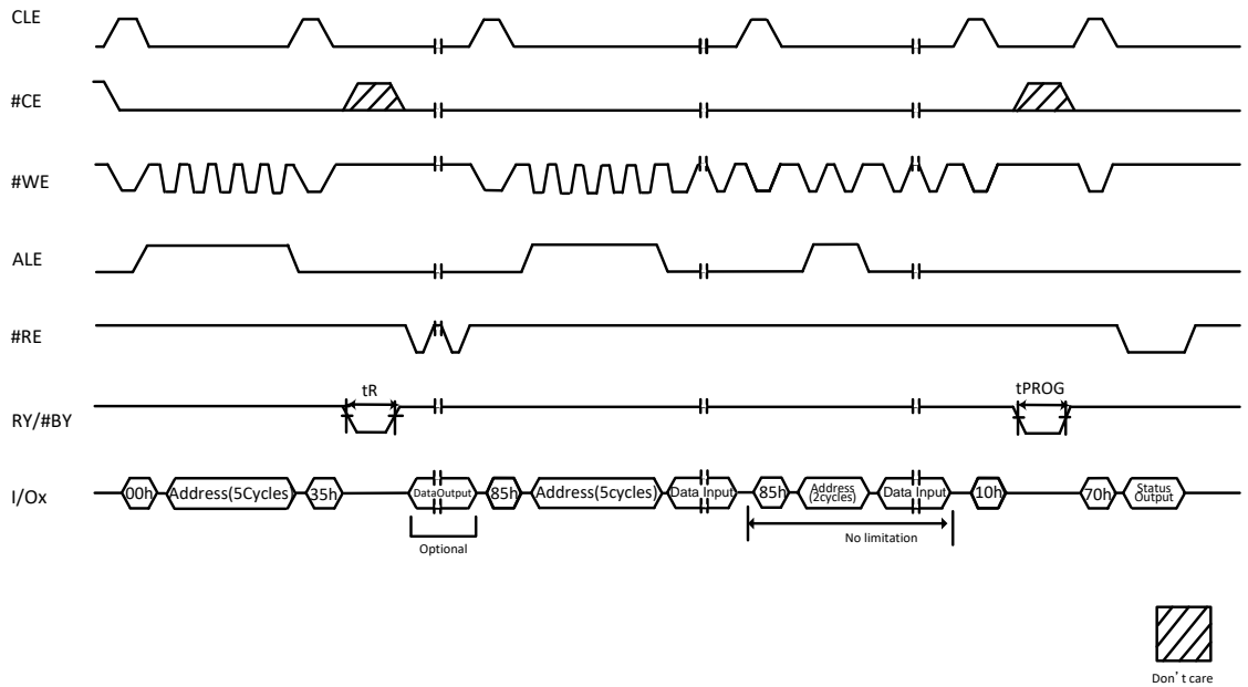
Figure 9-13 Copy Back Operation with Random Data Input
